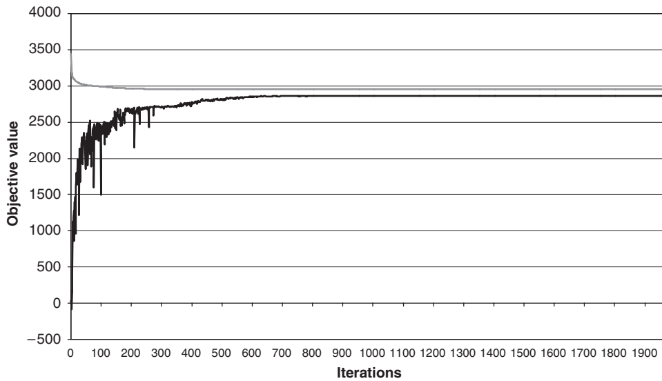
Fig. 5. ColGen(t) with augmentation: LB = 2862.21.
