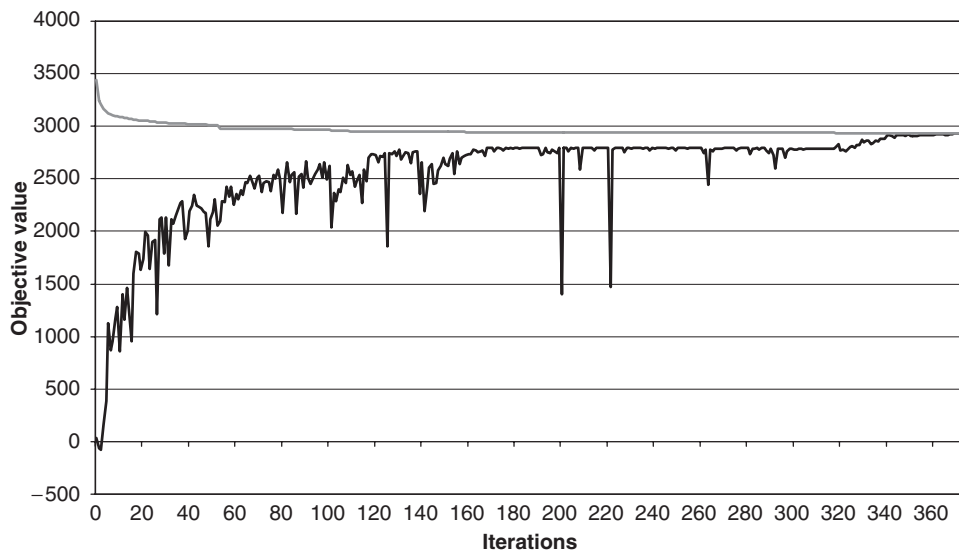
Fig. 6. ColGen(t) with augmentation and controlled perturbation: LB = 2936.49.
